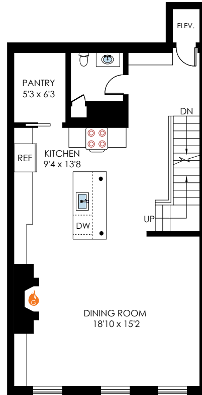
MAIN LEVEL 689 FIN. SQ. FT. 9' CEILING
