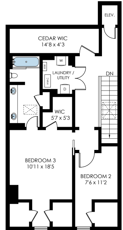
UPPER LEVEL 2 689 FIN. SQ. FT. 8' CEILING
